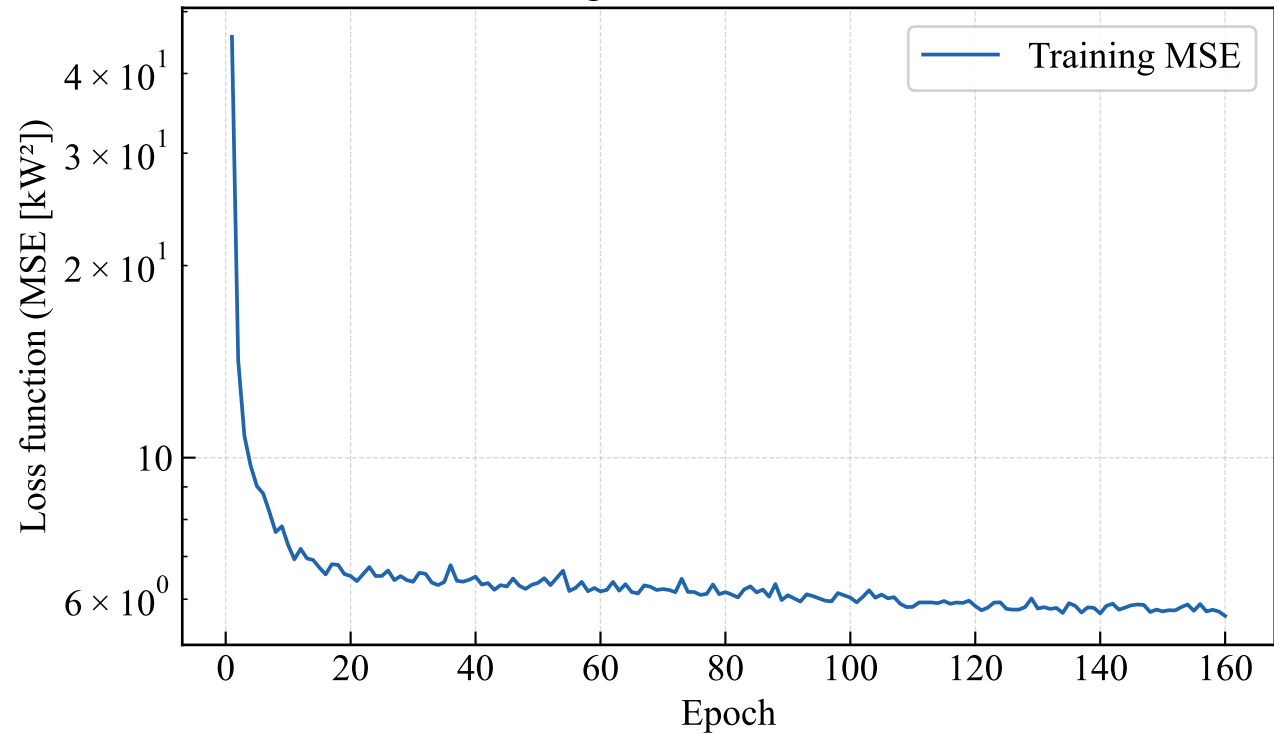
Learning curve — LSTM model
